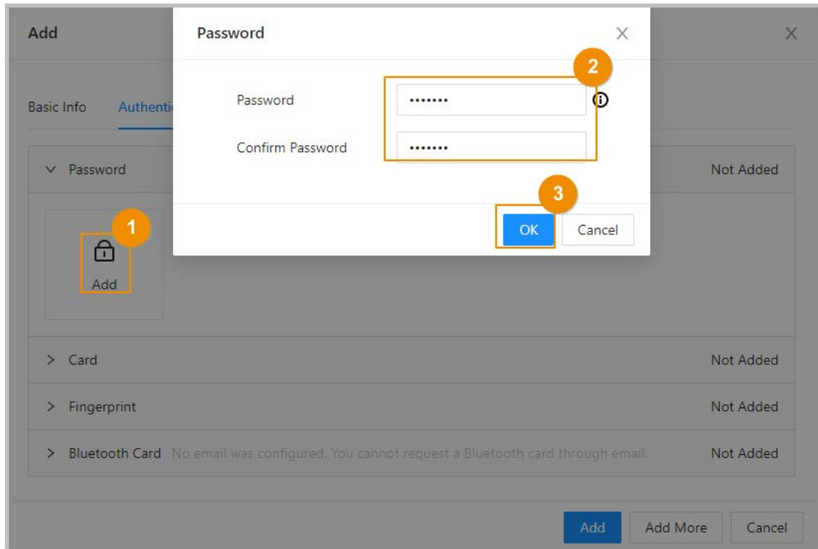
Figure 5-14 Add password
