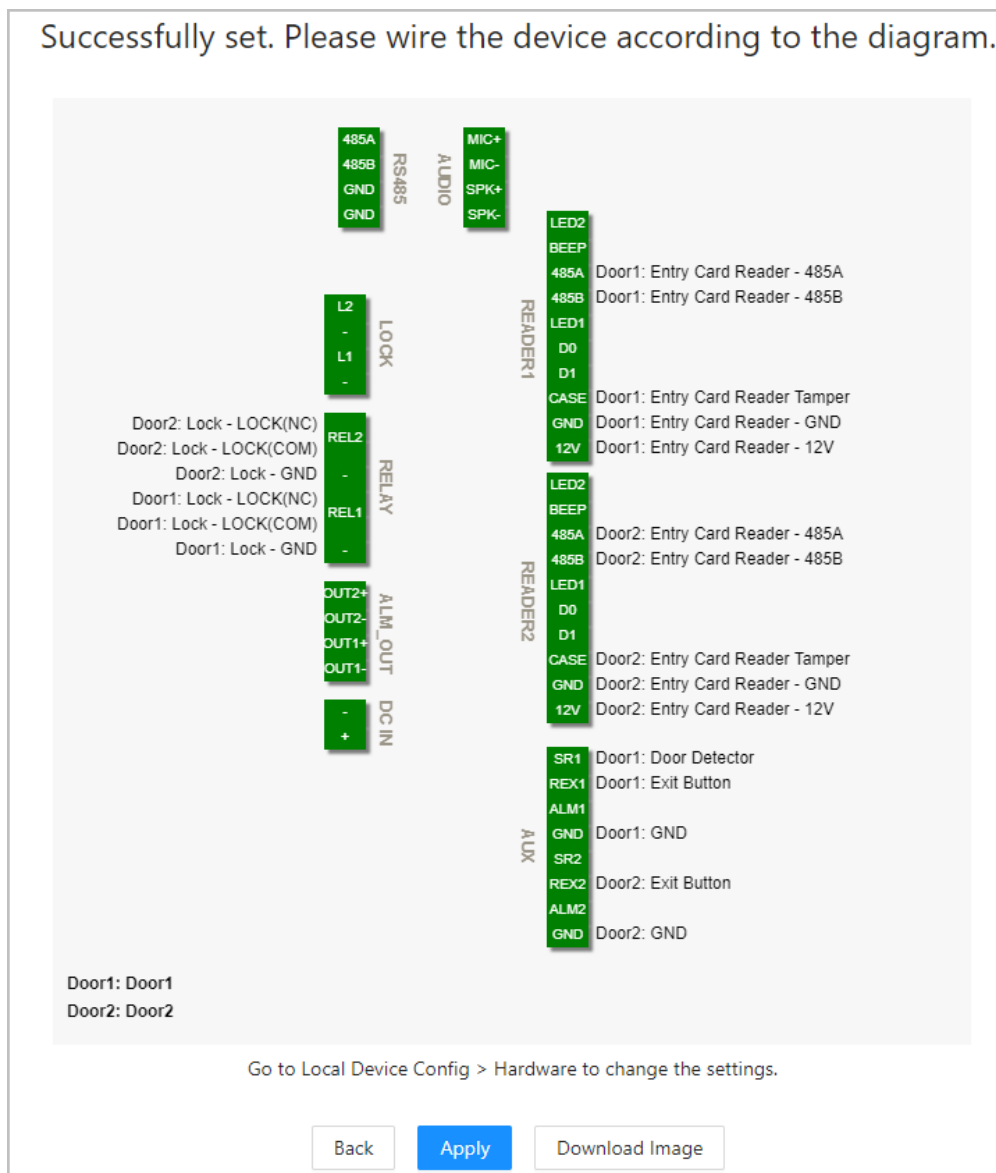
Figure 5-8 Wiring diagram
