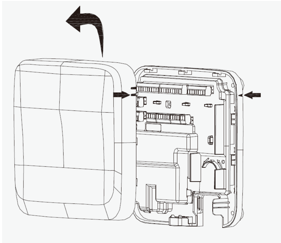
Figure 4-2 Remove the front panel
