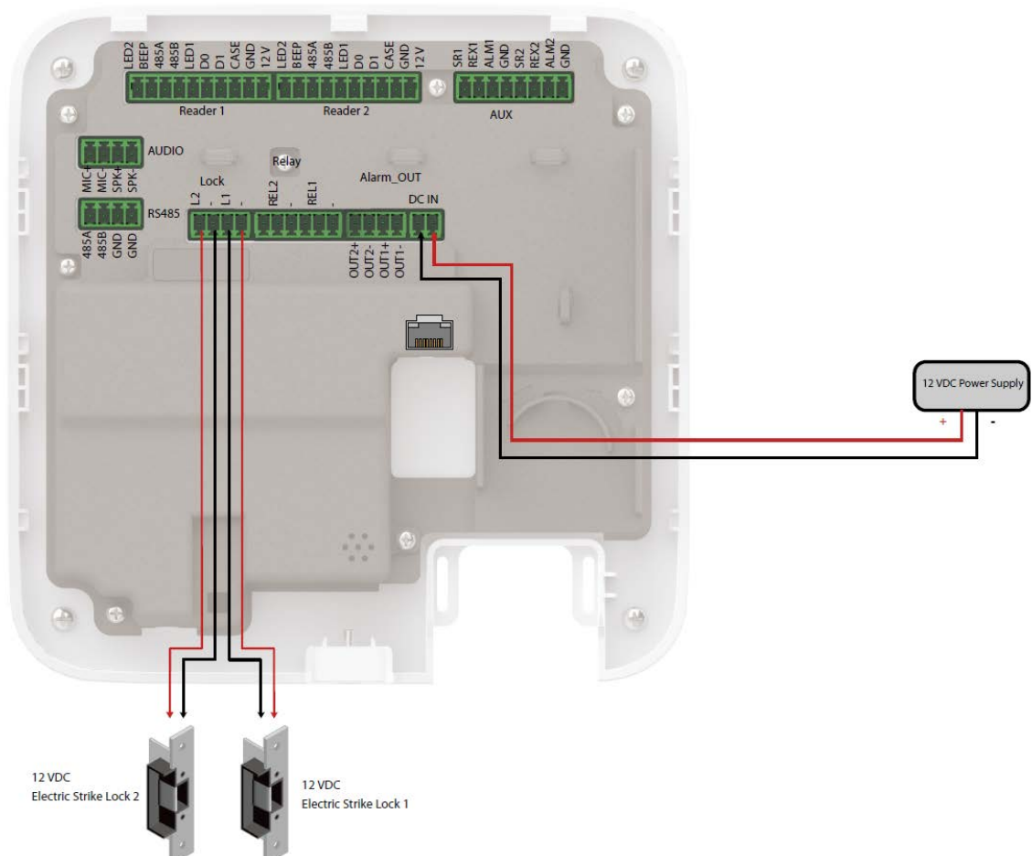
Figure 3-18 Wiring of locks
